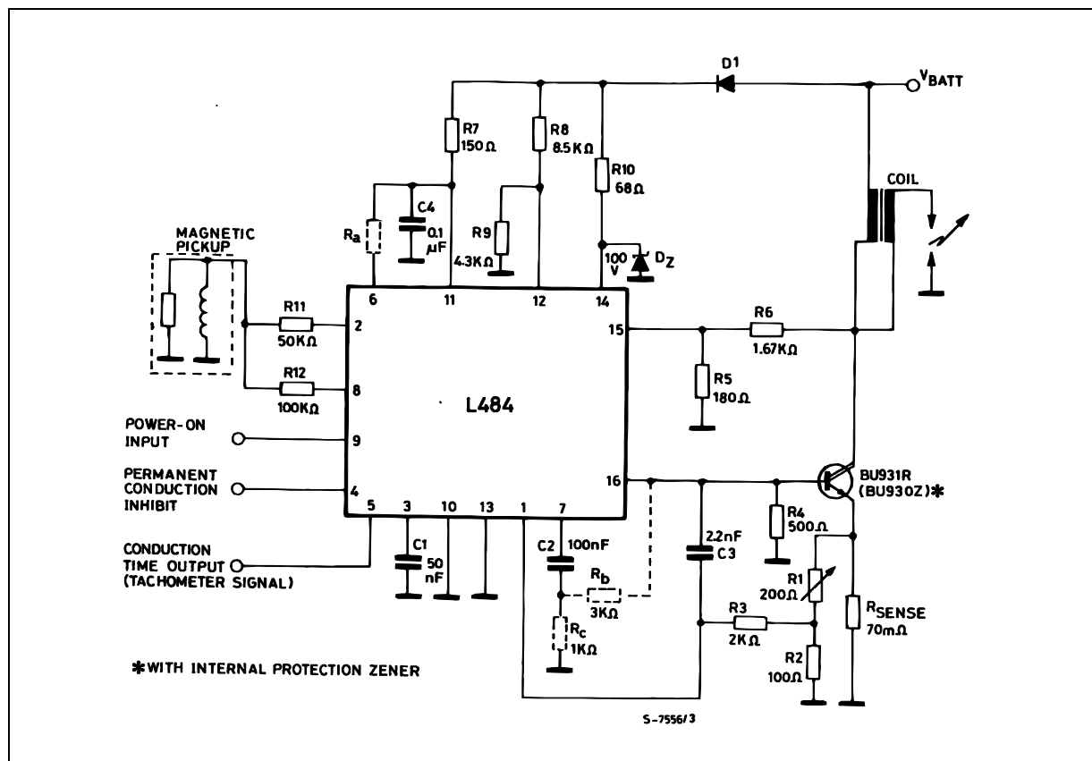
Figure 2 : Application Circuit.
